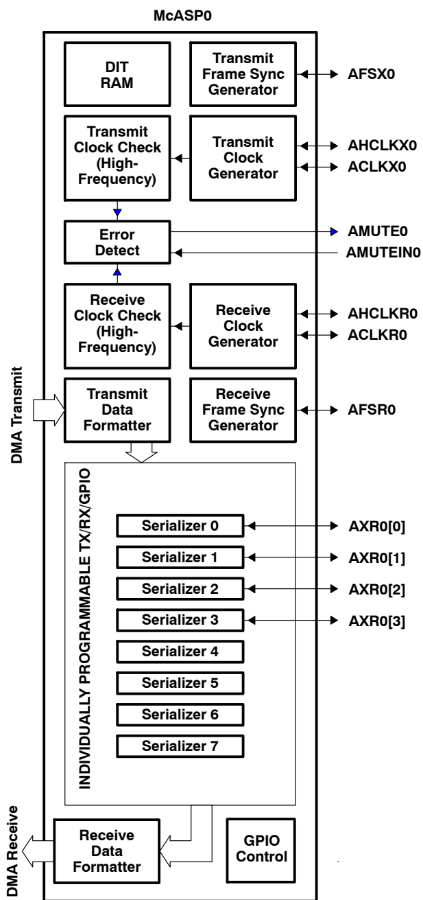
Figure 4-34. McASP0 Configuration
