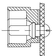
DETAIL P (INSTALLED IN PCB, SEE NOTE 6)
