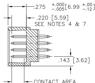
SECTION X-X
