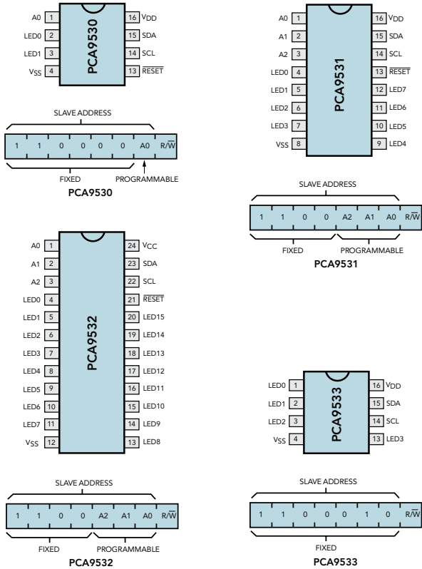
Pin configurations
