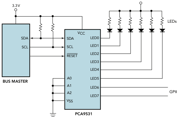
Typical application
