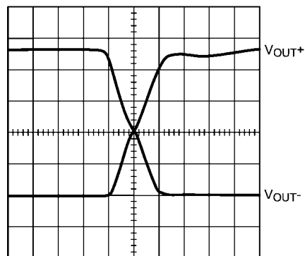
Output Transition High to Low, Low to High V_{DD} = 5V , 1V/div, 1 \mu s/div
