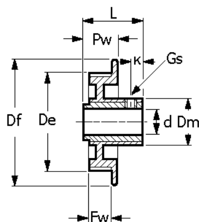
Type C with Brass Insert
