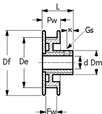
Type B with Aluminium Insert
