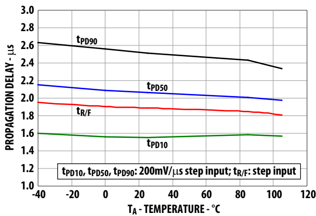
Figure 19. Propagation delay, output rise/fall time vs. temperature.
