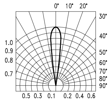
■ Directivity
