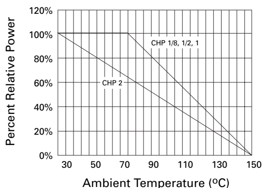
CHP Power Derating Curve
