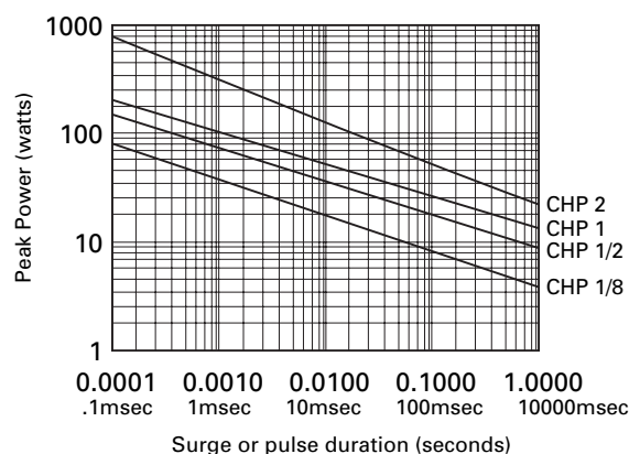
CHP Repetitive Surge Curve
