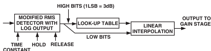
Figure 10. Gain Derived from Interpolated Look-Up Table
