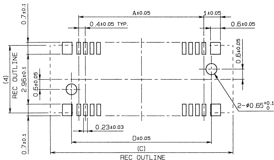
MOUNTING LAYOUT
