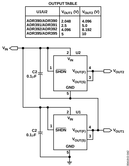
Figure 42. Stacking Voltage References with the ADR390/ADR391/ADR392/ADR395
