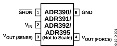
Figure 1. 5-Lead TSOT (UJ Suffix)
