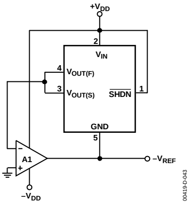
Figure 43. Negative Reference
