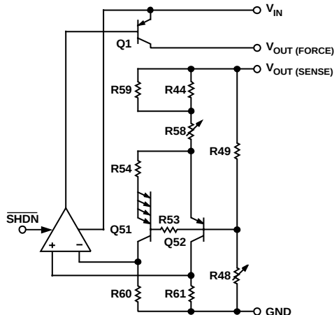
Figure 40. Simplified Schematic
