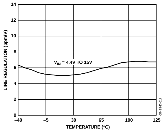
Figure 17. ADR392 Line Regulation vs. Temperature
