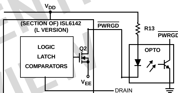
FIGURE 35. ACTIVE LOW ENABLE OPTO-ISOLATOR
