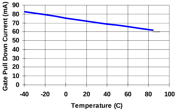
FIGURE 19. GATE PULL-DOWN CURRENT (UV/IOV/TIME-OUT) VS TEMPERATURE
