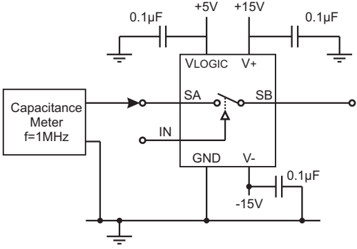
Figure 8 - Off Capacitance
