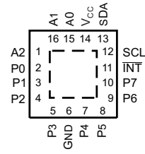
RGT PACKAGE (TOP VIEW)
