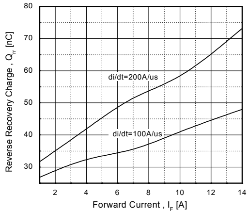
Figure 19. Stored Charge
