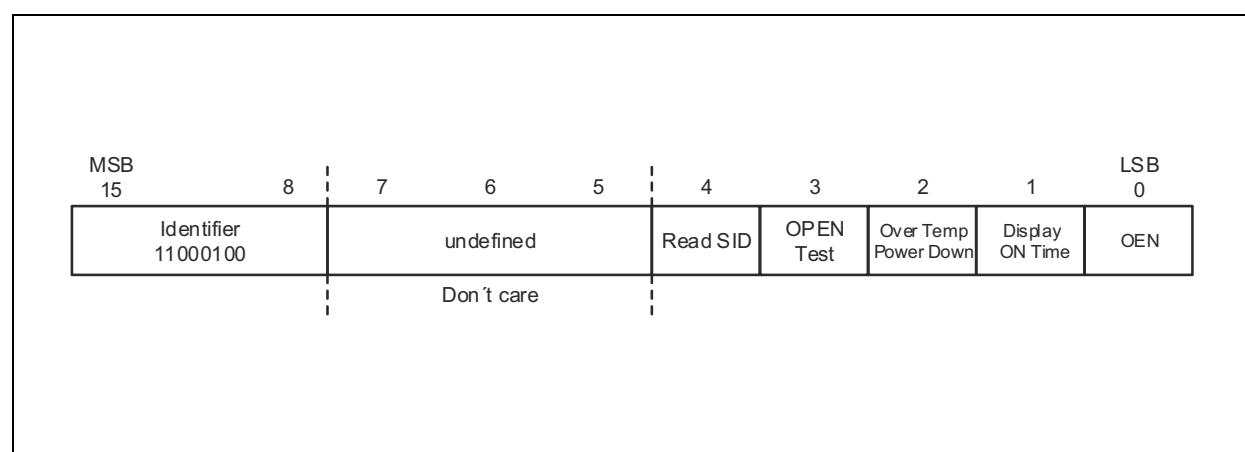
Figure 33: Command Packet Format
