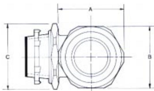
TYPE HKL— 90° CONNECTOR
