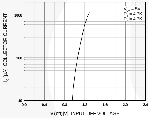
Figure 3. Input-Off Voltage
