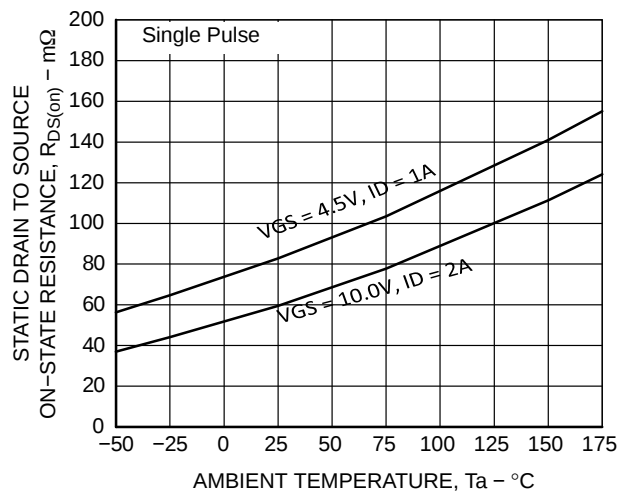
Figure 5. R_{DS(on)} - T_a
