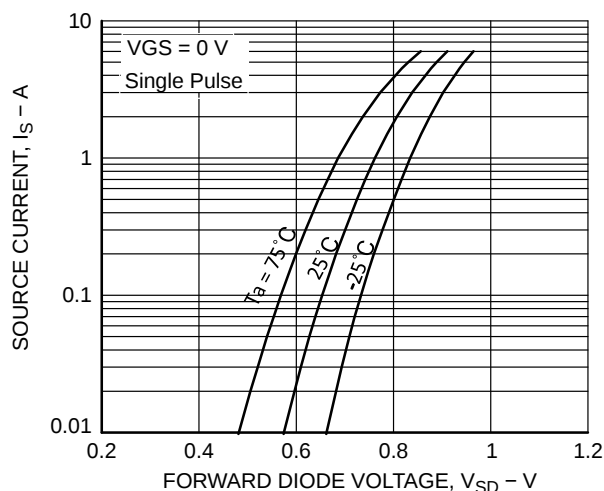
Figure 7. I_S - V_{SD}
