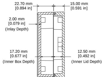
SECTION A-A END VIEW OF ASSEMBLY
