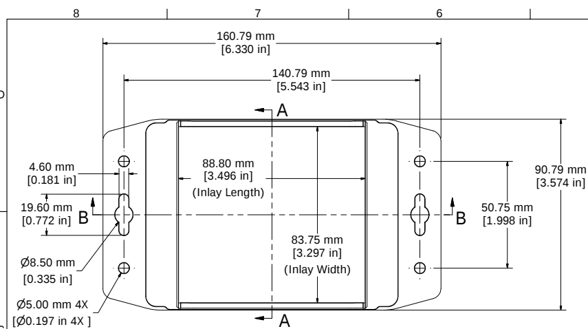
ENCLOSURE ASSEMBLY TOP VIEW
