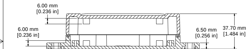
SECTION B-B (SIDE VIEW OF ASSEMBLY)
