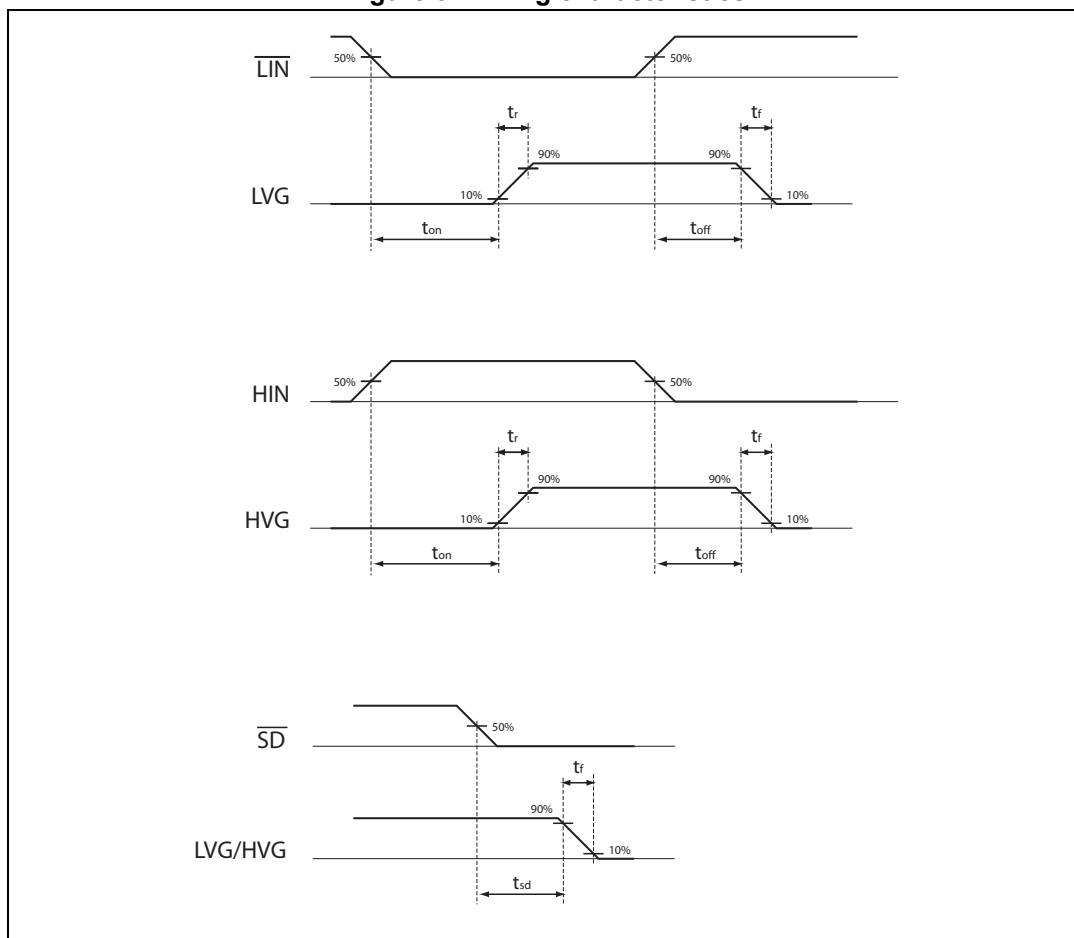
Figure 3. Timing characteristics
