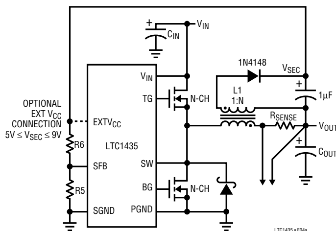
Figure 4a. Secondary Output Loop and EXT V CC Connection
