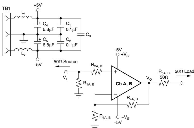
Figure 2. Schematic for DEM-OPA-SO-2B
