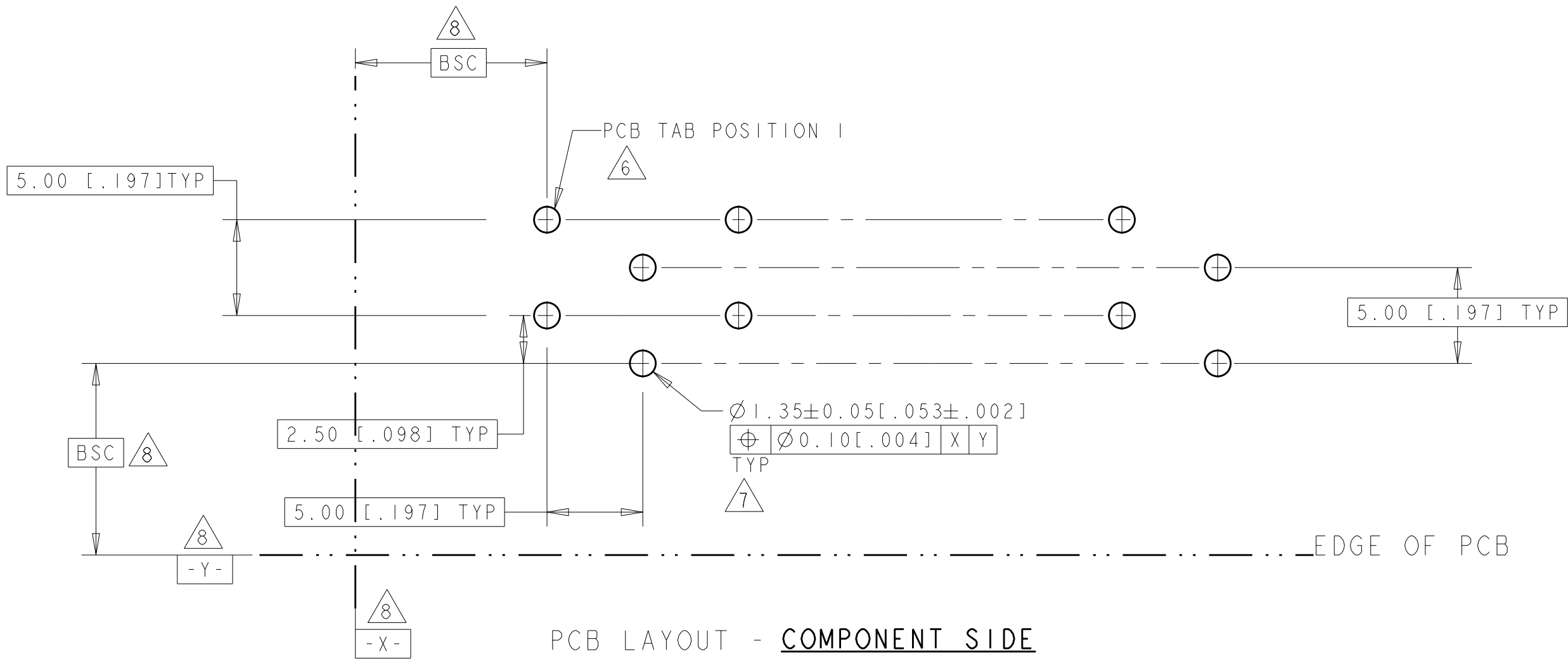
PCB LAYOUT - COMPONENT SIDE PCB 1.5±0.14 [.059±.006] THICK SCALE 4:1
