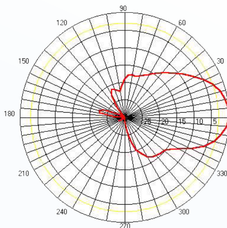
ES24-14 E-Plane at 2.4 GHz
