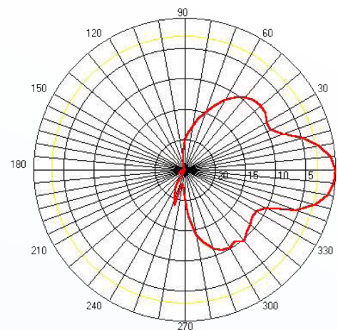
ES24-14 H-Plane at 2.4 GHz
