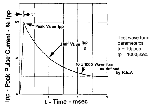
FIGURE 2 – PULSE WAVEFORM
