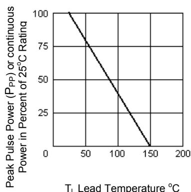
FIGURE 3 – Derating Curve
