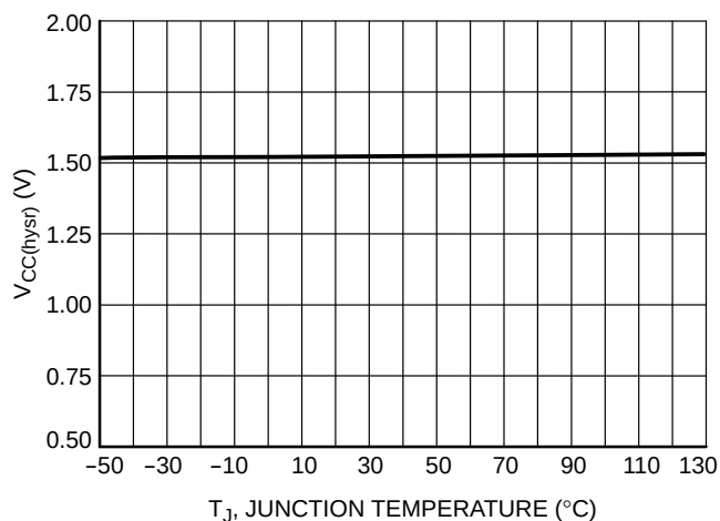
Figure 8. Hysteresis ( V_{CC(on)} - V_{CC(off)} ) vs. Temperature (A, A1, A2 and A3 Versions)
