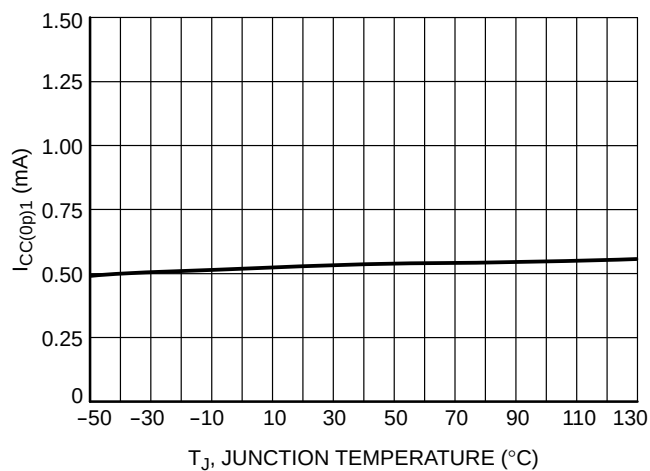
Figure 10. Operating Current, No Switching ( V_{SENSE} Grounded) vs. Temperature
