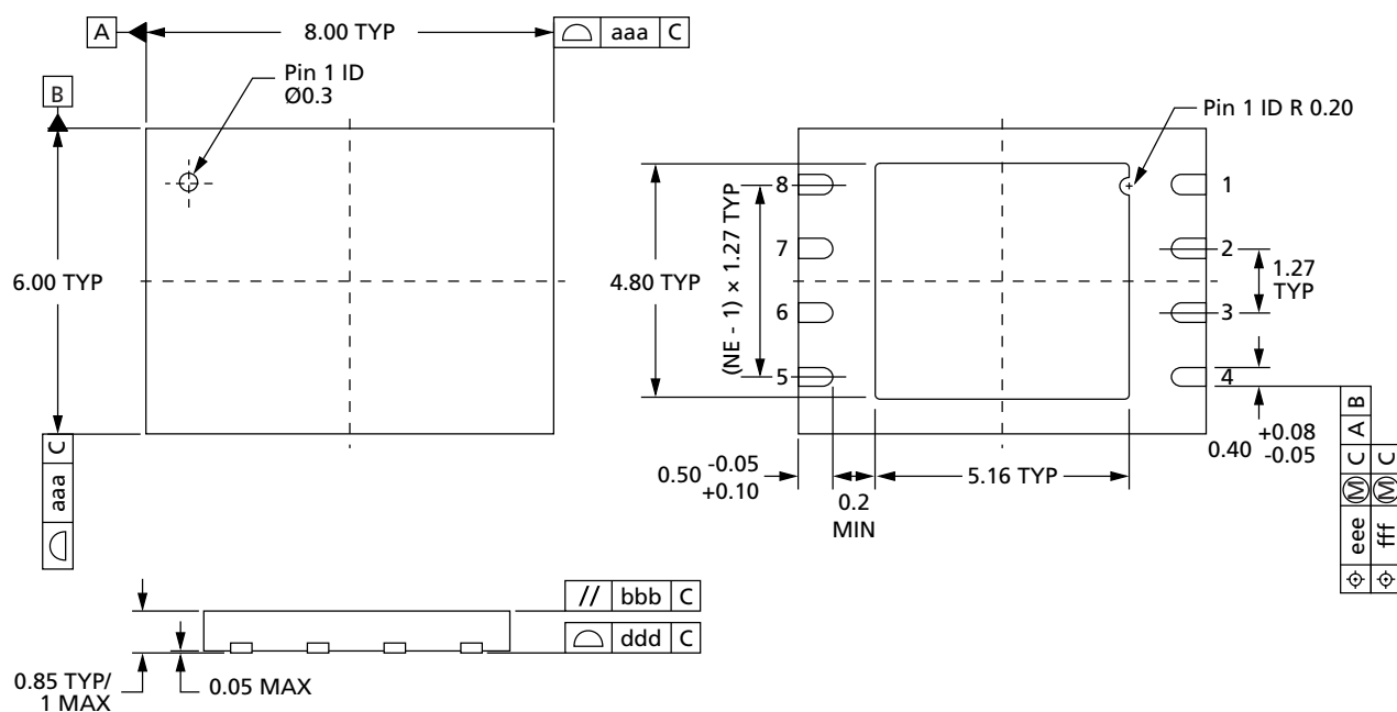
Figure 42: V-PDFN-8 8mm x 6mm (MLP8) – Package Code: F8
