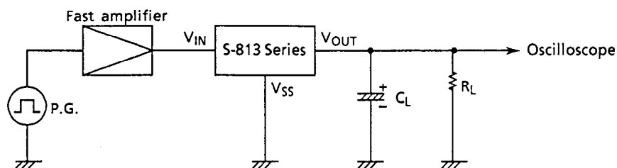
Figure 9 Measuring circuit
