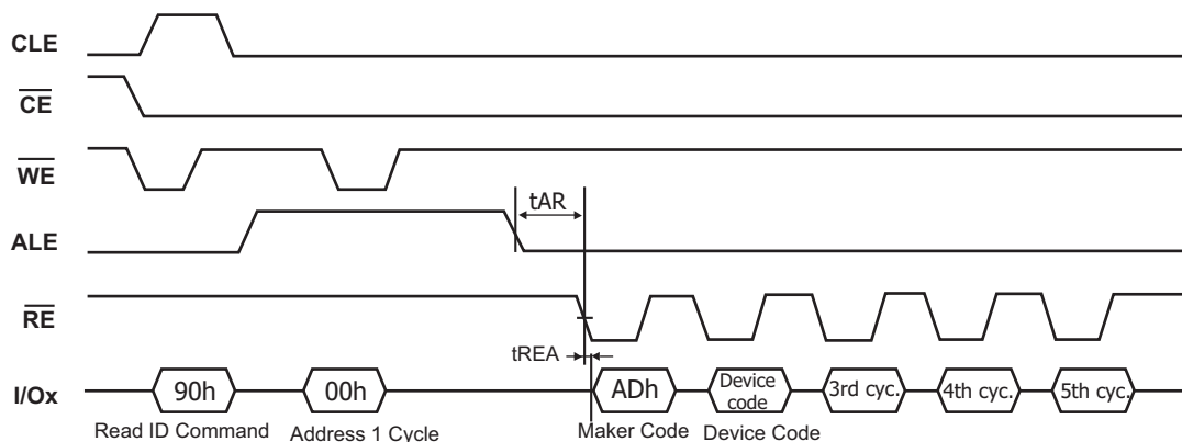
Figure 27: ID Read
