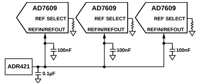
Figure 39. Single External Reference Driving Multiple AD7609 REFIN/REFOUT Pins
