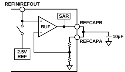
Figure 38. Reference Circuitry
