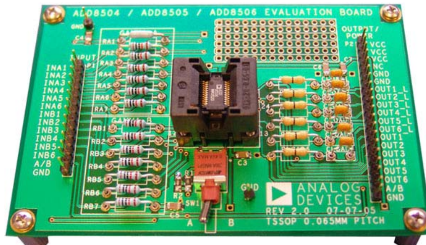
Figure 1. ADD8504/ADD8505/ADD8506 Evaluation Board
