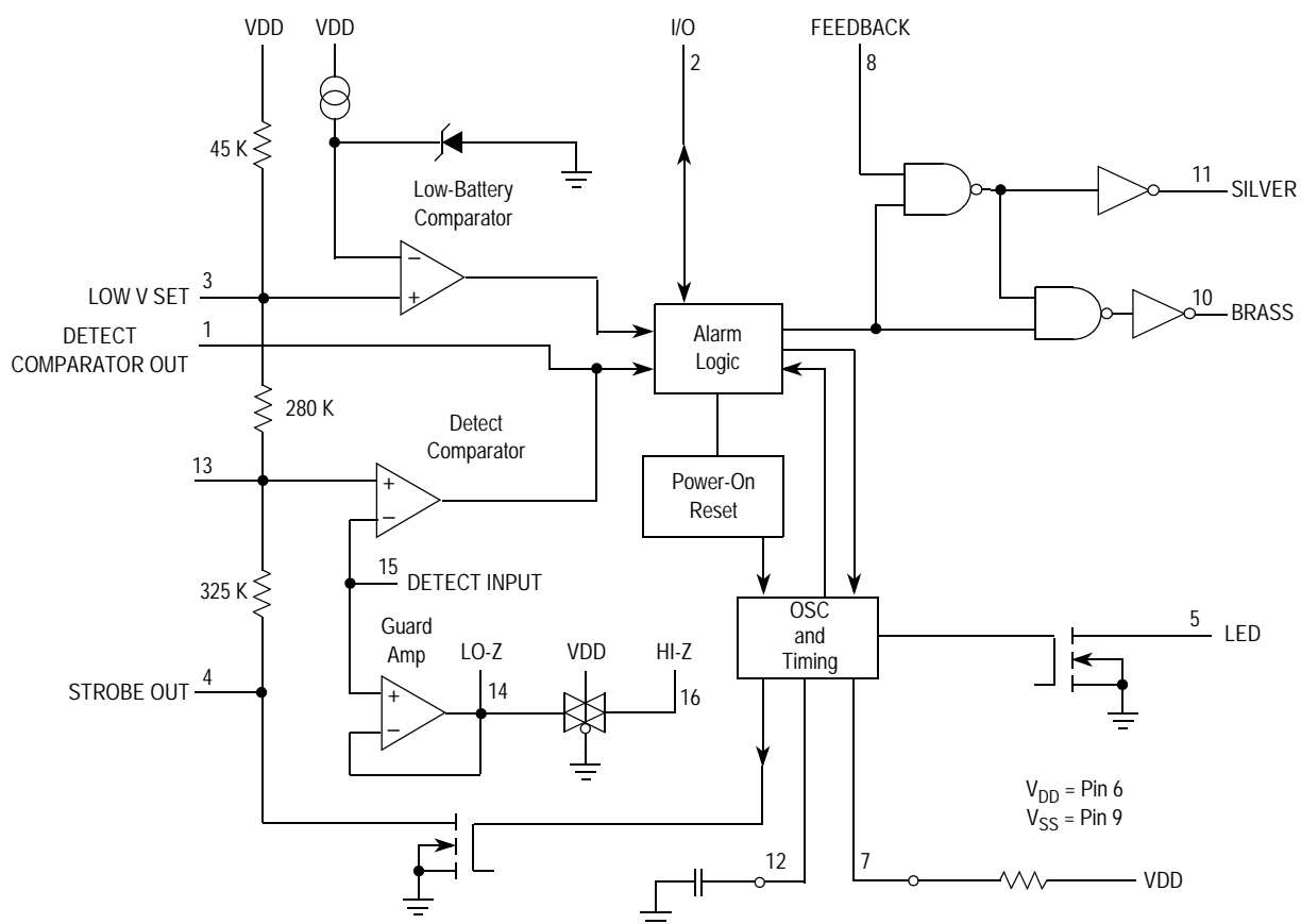
Figure 2. Block Diagram
