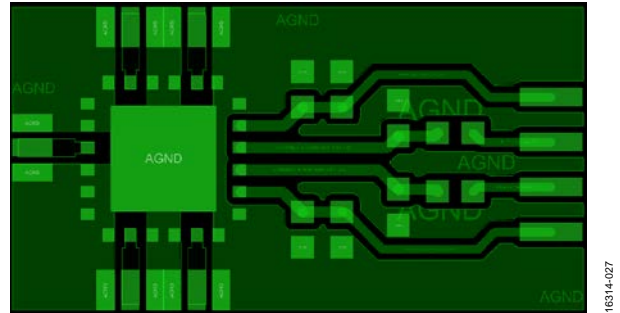
Figure 27. Probe Board Layout (Top View)
