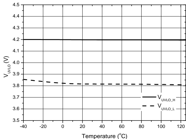
V_{UVLO} vs. Temperature (AL5816)
