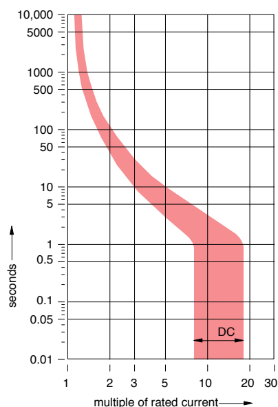
Tripping characteristic K
