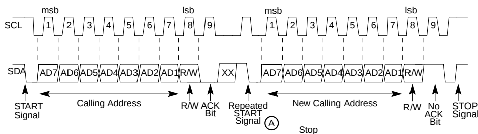
Figure 8-3. Repeated START
