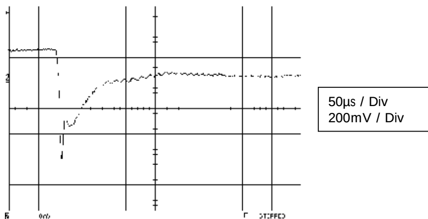
Figure 3 Output voltage transients Egston Power Supply N2GFSW 24W 15V representative sample, 10% to 100% resistive load change at 1kHz
