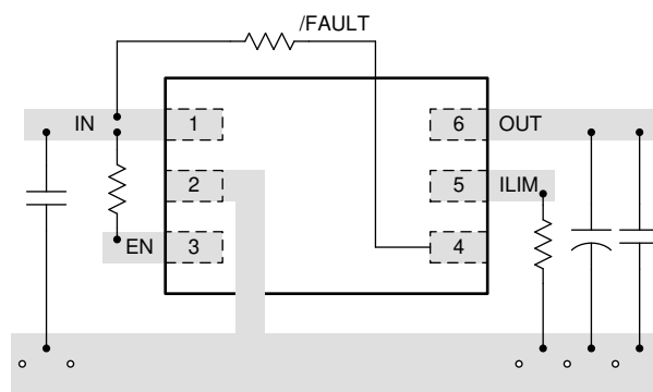
Figure 10-6. Layout Recommendation
