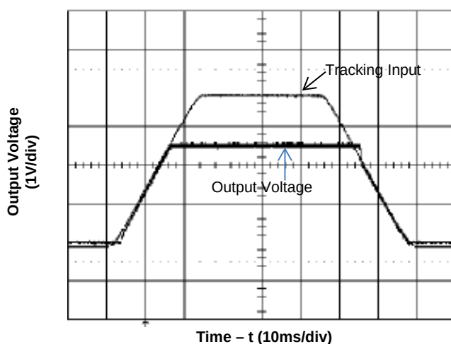
Figure 9. Voltage Tracking/Sequencing (voltage tracking option, V_{in}=12V , V_o=2.5V , I_o=0A )
