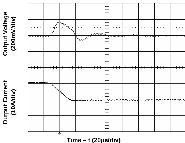
Figure 10. Transient Load Response (typical V_{in} , load current steps from 100% to 50% at a slew rate 0.5A/µs)
