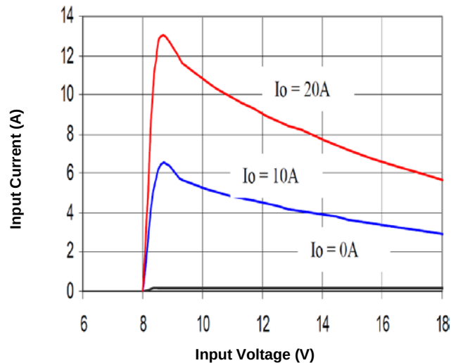
Figure 7. Input Characteristic ( V_o=5V )
