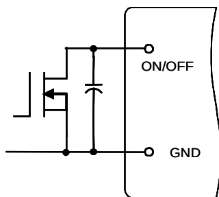
Figure 13. Circuit for Positive Logic Control
