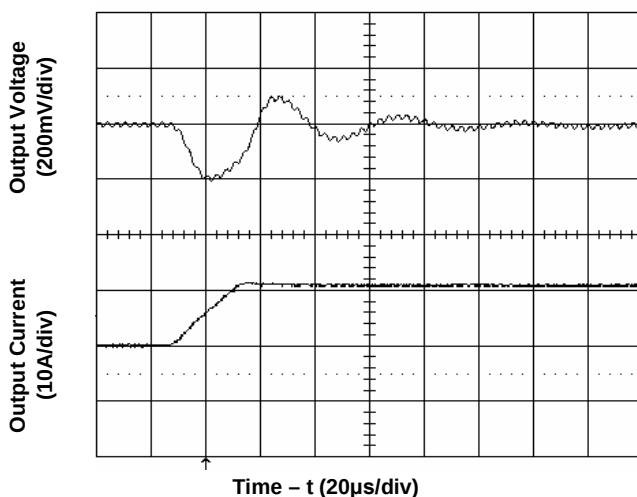
Figure 11. Transient Load Response (typical V_{in} , load current steps from 50% to 100% at a slew rate 0.5A/µs)
