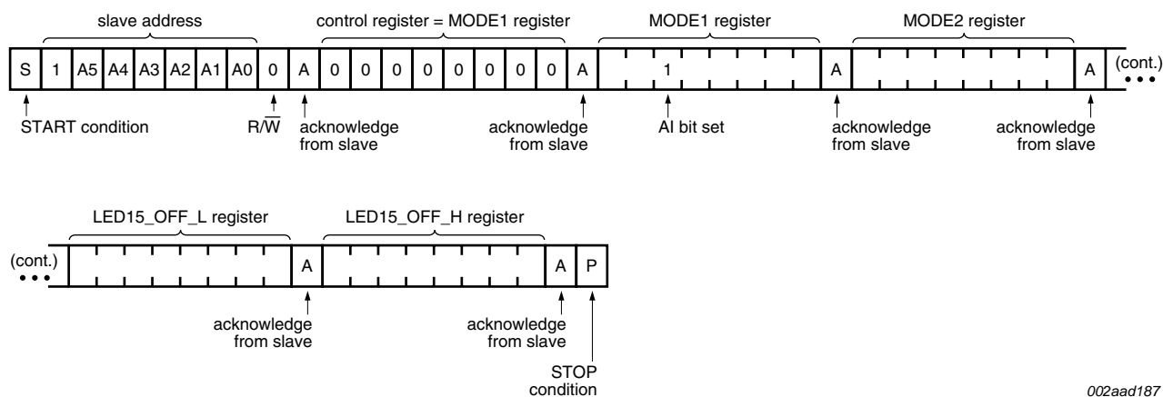
Fig 21. Write to all registers using the Auto-Increment feature; AI initially clear
