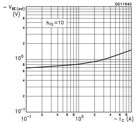
Base-Emitter Saturation Voltage
