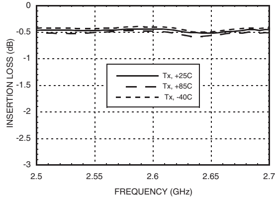
Insertion Loss vs. Temperature, Tx with 2600 MHz Tuning
