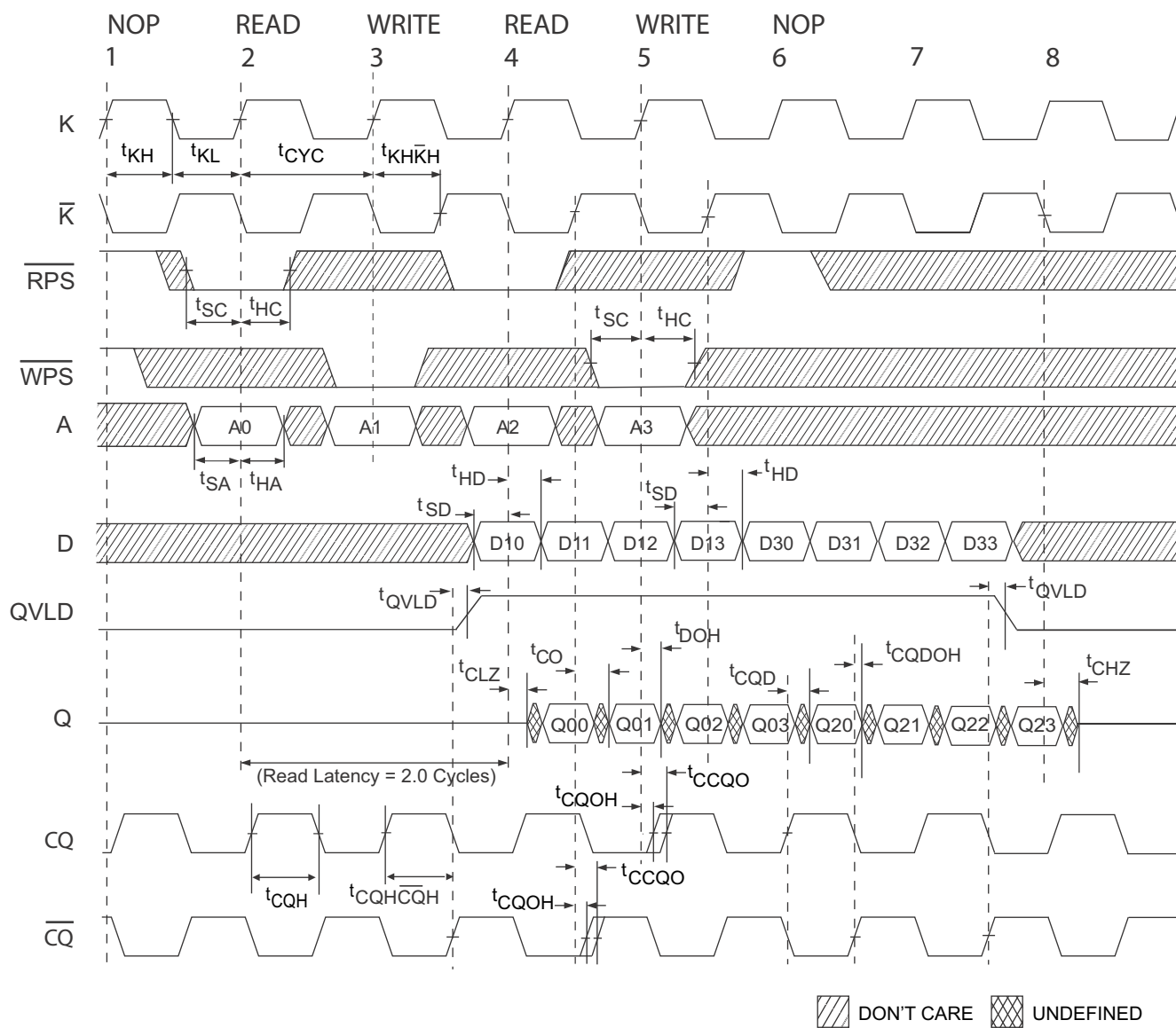
Figure 6. Read/Write/Deselect Sequence [38, 39, 40]
