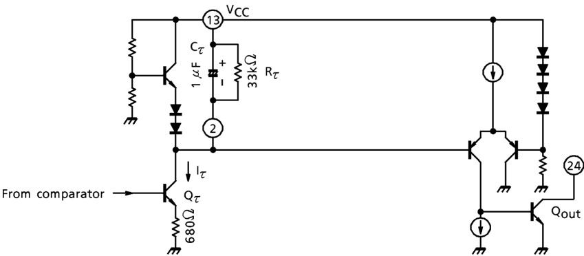
Fig.8 Output stage
