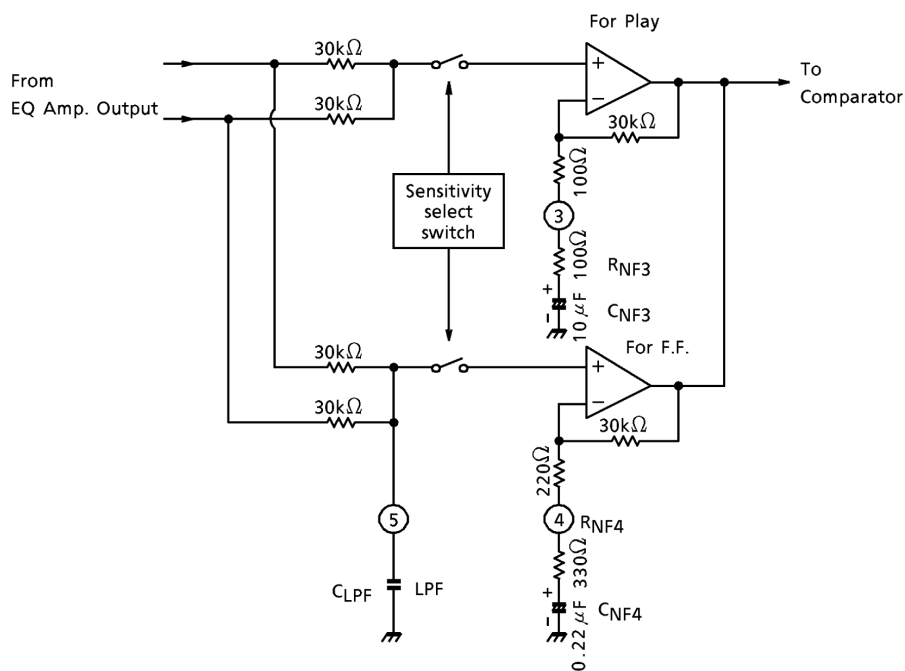
Fig.6 Sensor amp.
