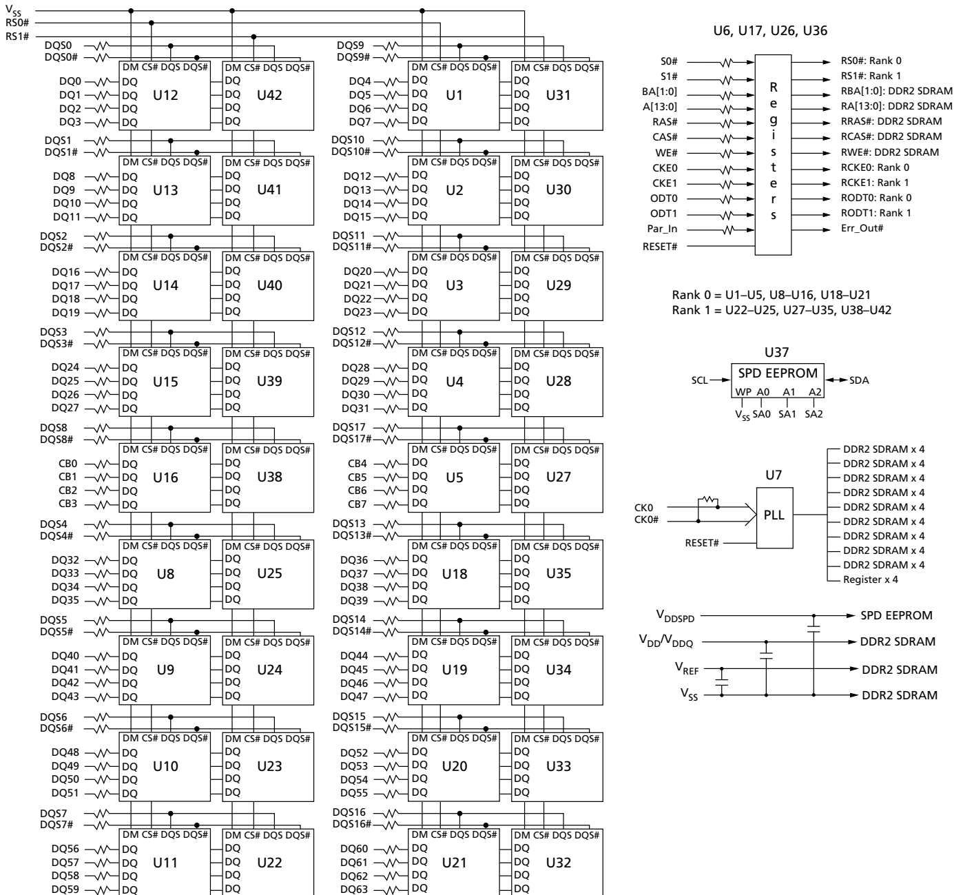
Figure 2: Functional Block Diagram – 2GB
