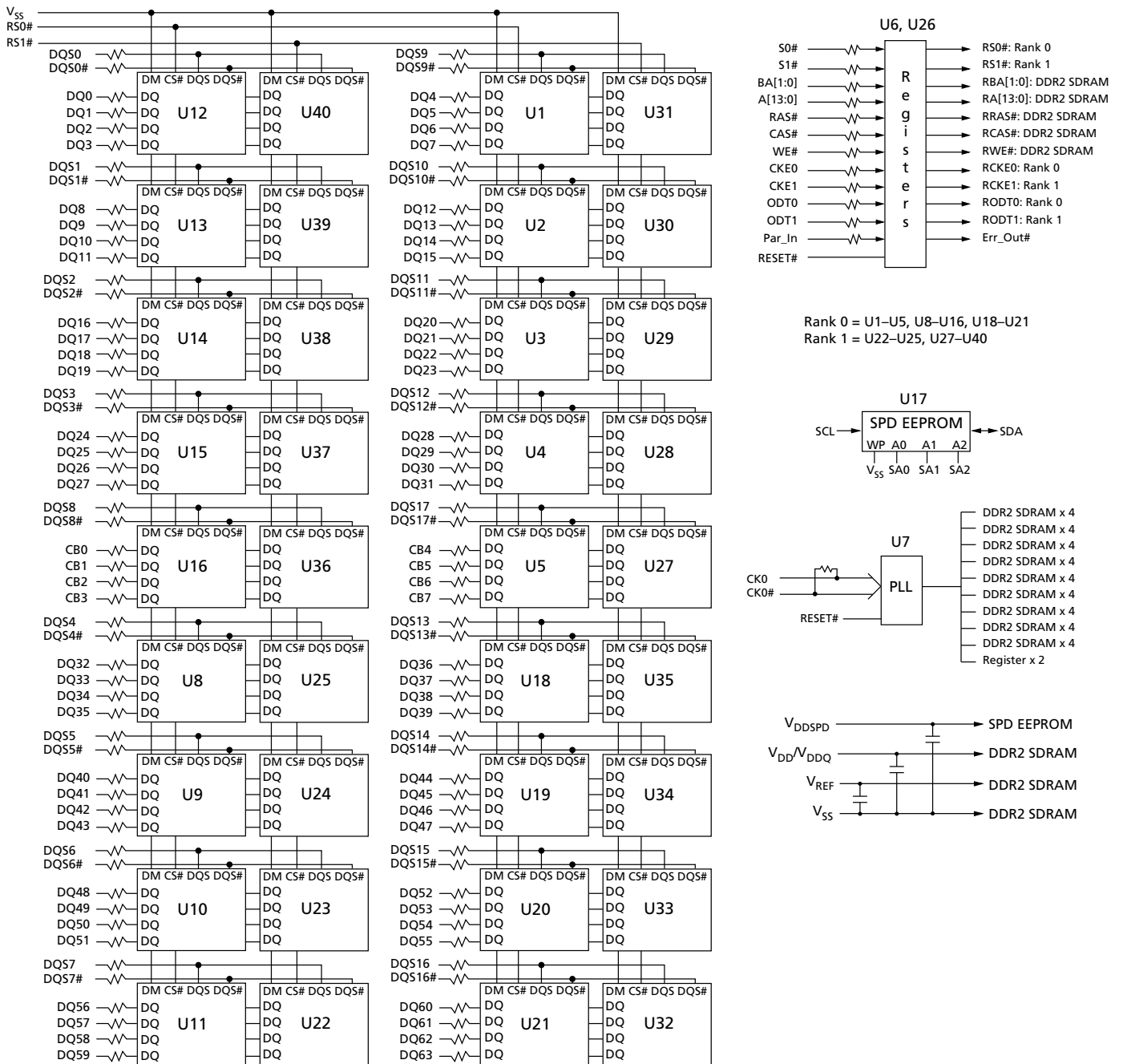
Figure 3: Functional Block Diagram – 4GB
