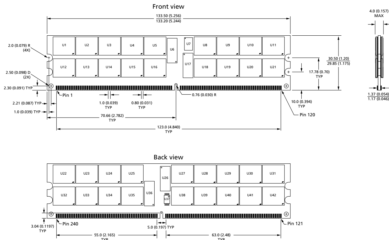
Figure 4: 240-Pin DDR2 RDIMM – 2GB
