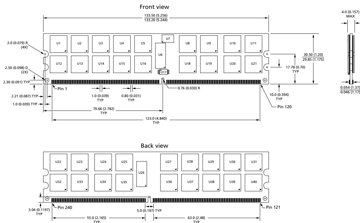
Figure 5: 240-Pin DDR2 RDIMM – 4GB
