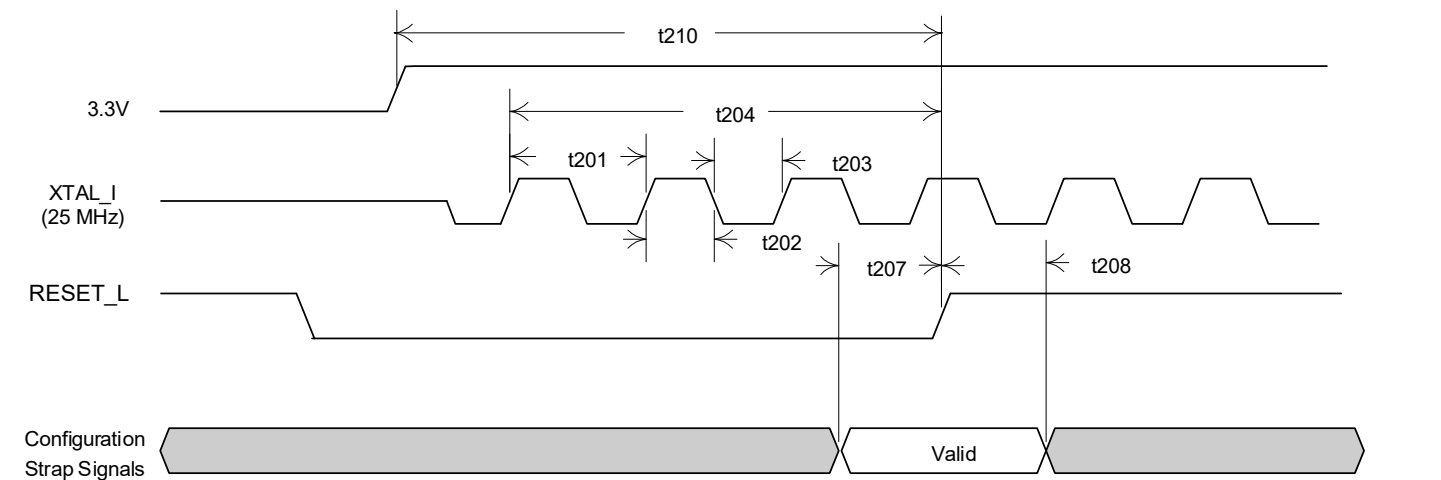
Figure 34: Reset and Clock Timing
