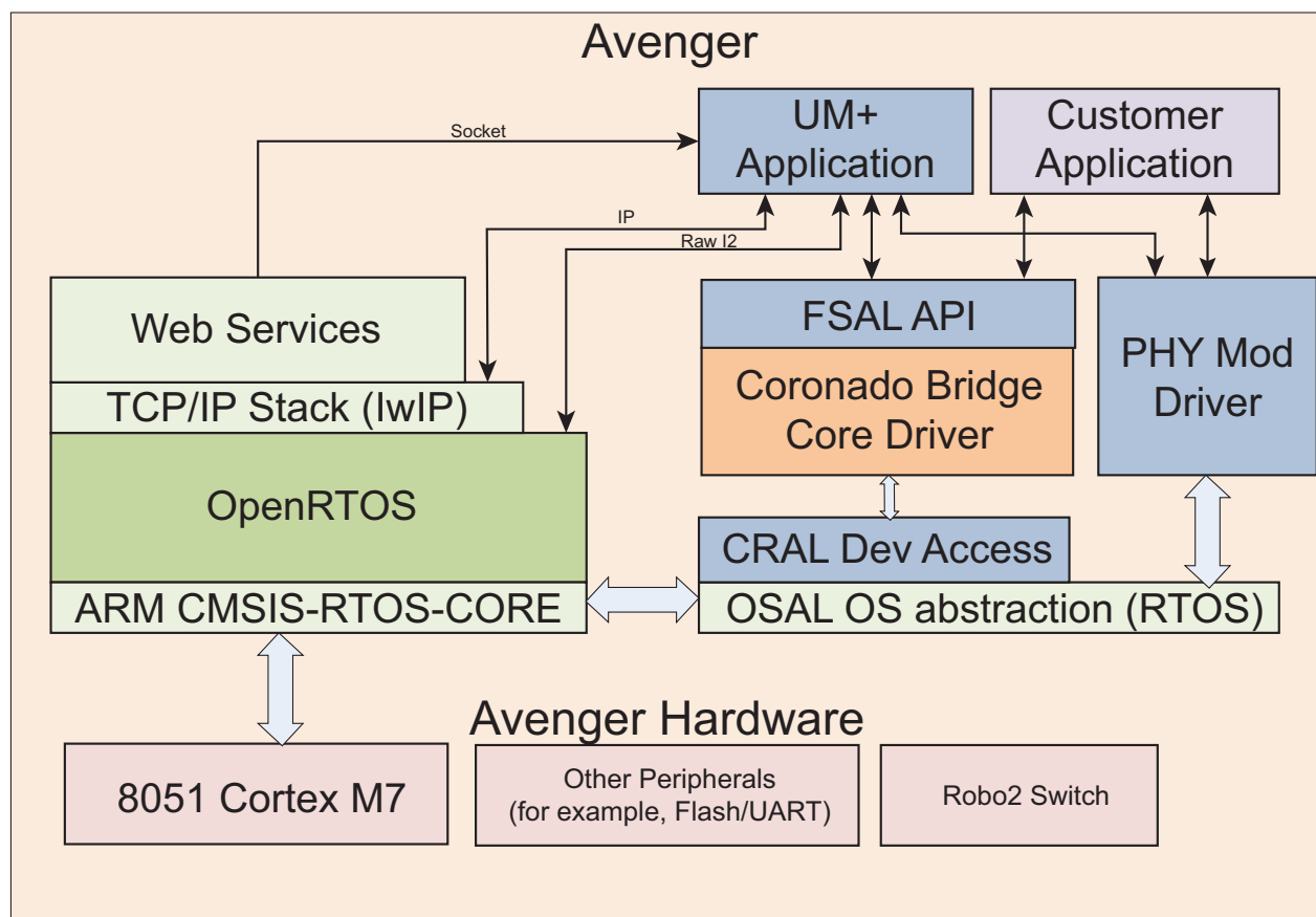
Figure 19: Web-Managed Application
