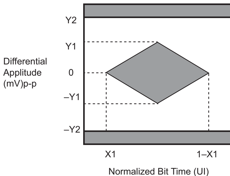
Figure 33: XFI Far-End Eye Mask
