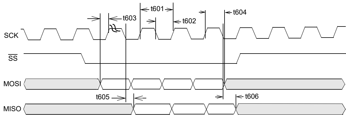
Figure 45: SPI-2 Timing, SS Asserted During SCK High
