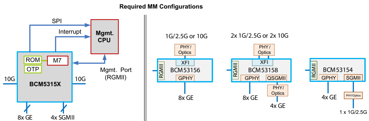
Figure 14: Managed Configurations
