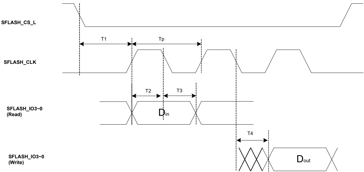
Figure 41: Serial Flash Timing Diagram
