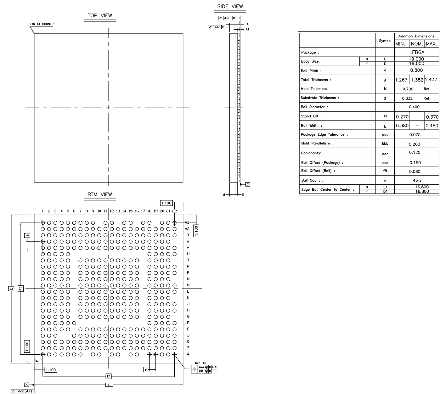
Figure 55: BCM53154 19×19 mm 2 Mechanical Information
