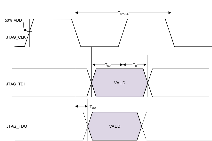
Figure 46: JTAG Interface
