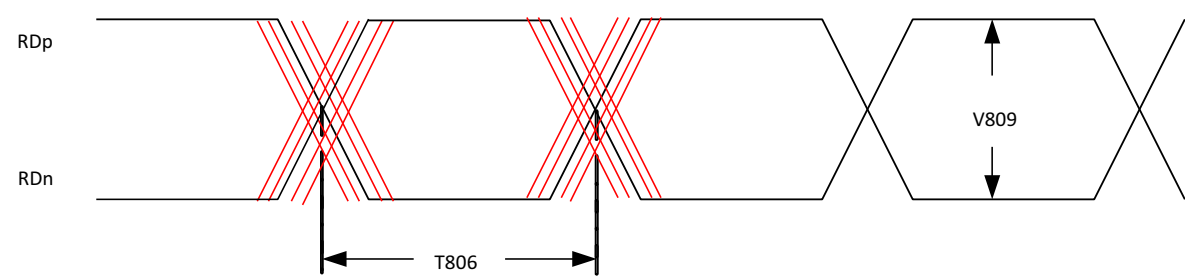
Figure 53: 2.5GE/SerDes Interface Input Timing
