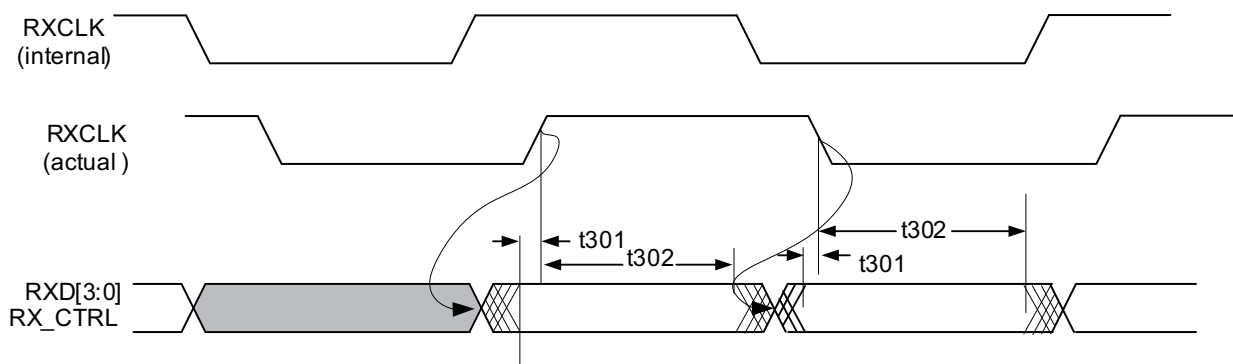
Figure 38: RGMII Input Timing (Delayed Mode)
