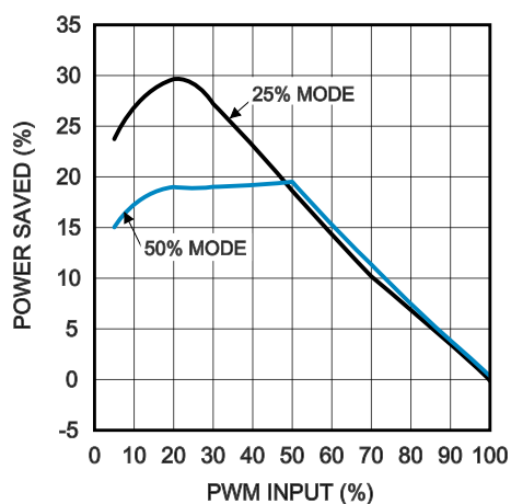
Power saved with PWM &amp; current mode compared to PWM mode
