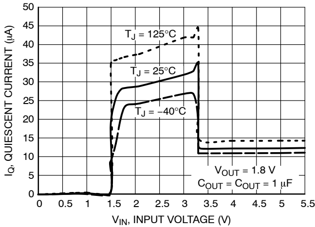
Figure 63. Quiescent Current vs. Input Voltage V_{OUT} = 1.8 V
