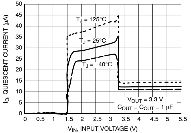
Figure 64. Quiescent Current vs. Input Voltage V_{OUT} = 3.3 V
