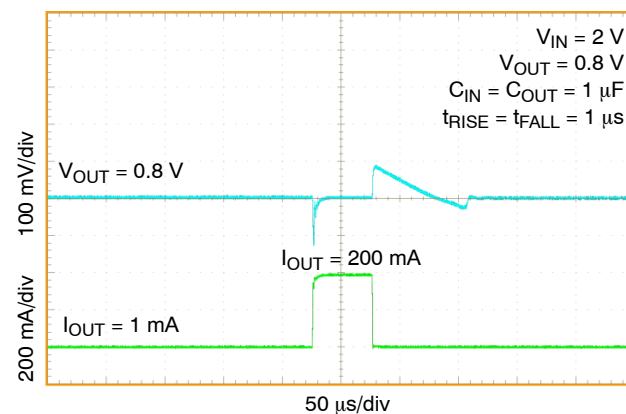
Figure 6. Load Transient Response, 1 mA – 200 mA NCV8752A/B, V_{OUT} = 0.8 V
