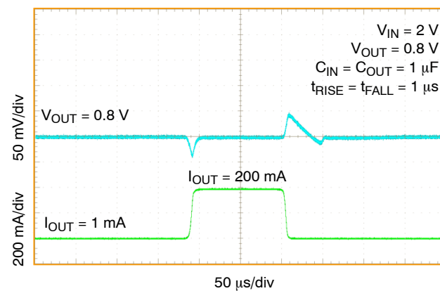
Figure 8. Load Transient Response, 1 mA – 100 mA NCV8752A/B, V_{OUT} = 0.8 V
