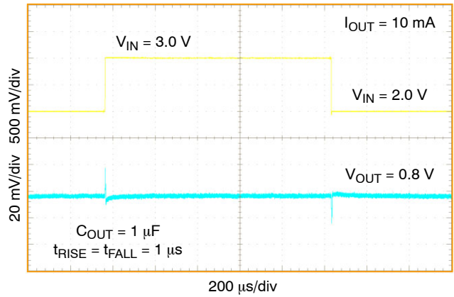
Figure 52. Line Transient 2 V – 3 V NCV8752A/B, V_{OUT} = 0.8 V
