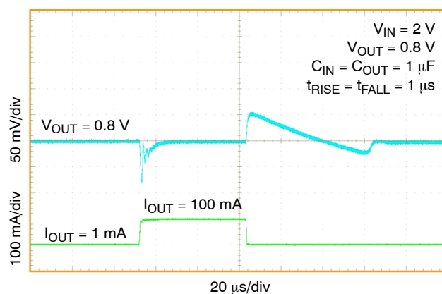
Figure 4. Load Transient Response, 1 mA – 100 mA NCV8752A/B, V_{OUT} = 0.8 V
