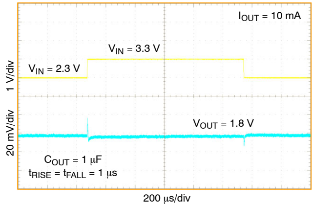
Figure 54. Line Transient 2.3 V – 3.3 V NCV8752A/B, V_{OUT} = 1.8 V
