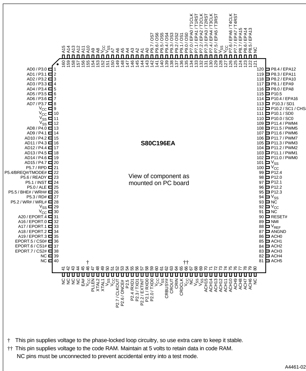
Figure 3. S80C196EA 160-pin QFP Package
